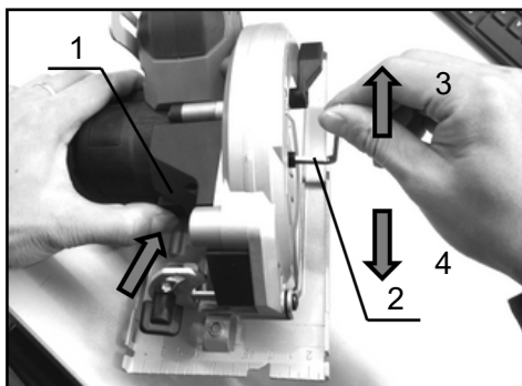
► 1. Shaft lock 2. Hex wrench 3. Loosen 4. Tighten
