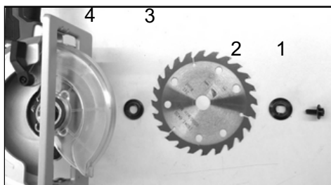
► 1. Hex bolt 2. Outer flange 3. Circular saw blade 4. Inner flange
