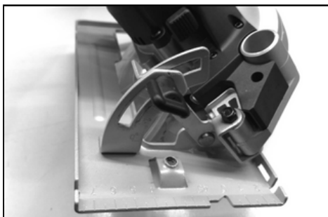
► 1. Cutting angle adjust lever 2. Base
