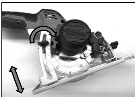
► 1. Cutting depth adjust clamping screw 2. Base
